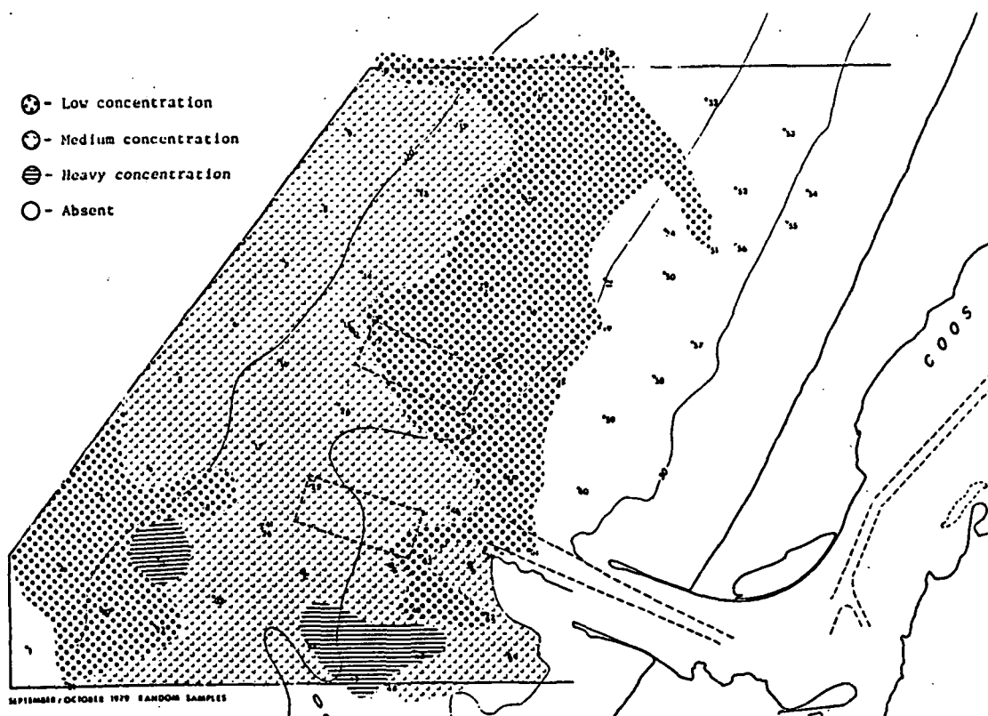
Figure 3.17 Distribution of wood chips; Cruise I & II, 1979 (from Hancock et al., 1981)
