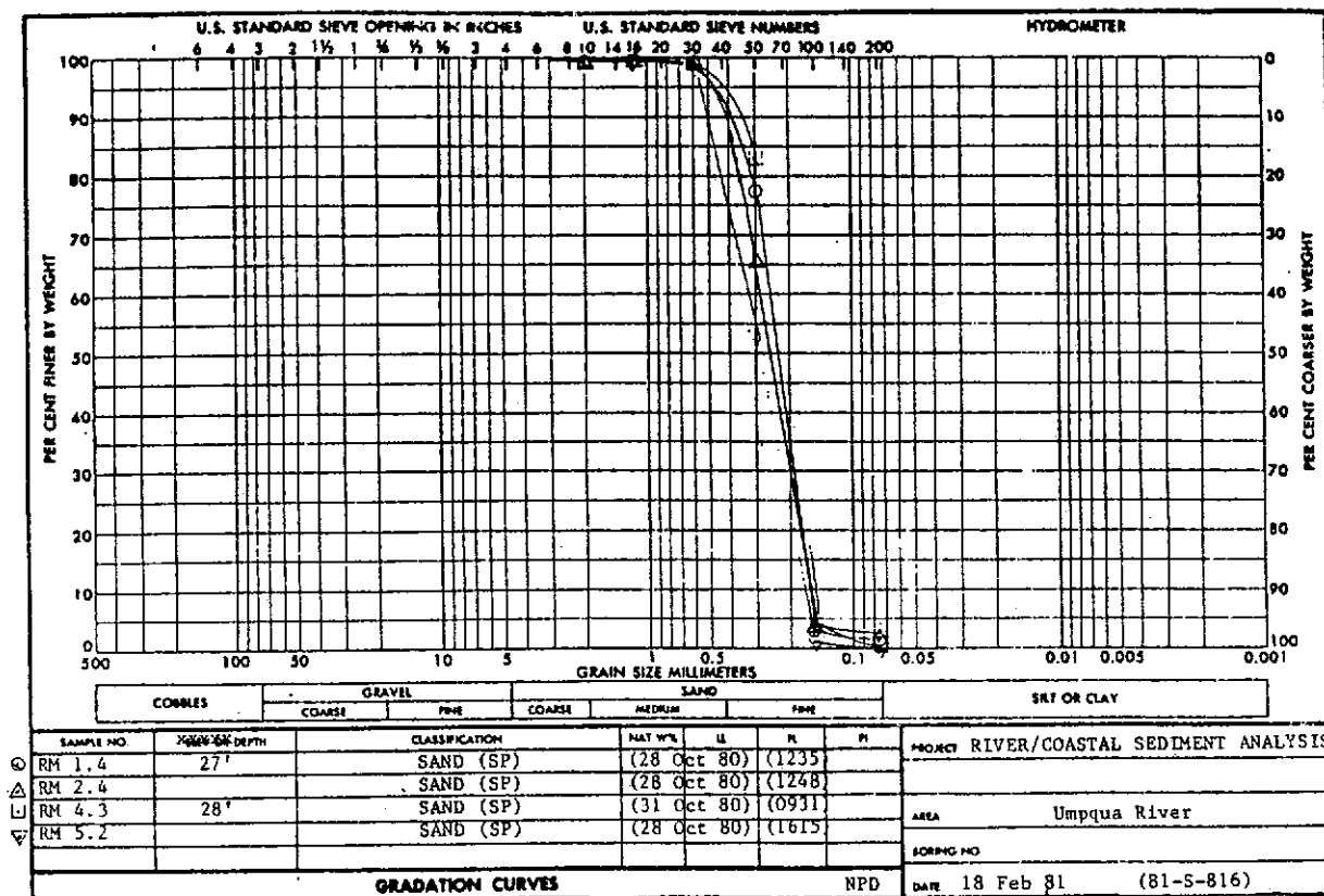
Figure C-6 Gradation Curves
