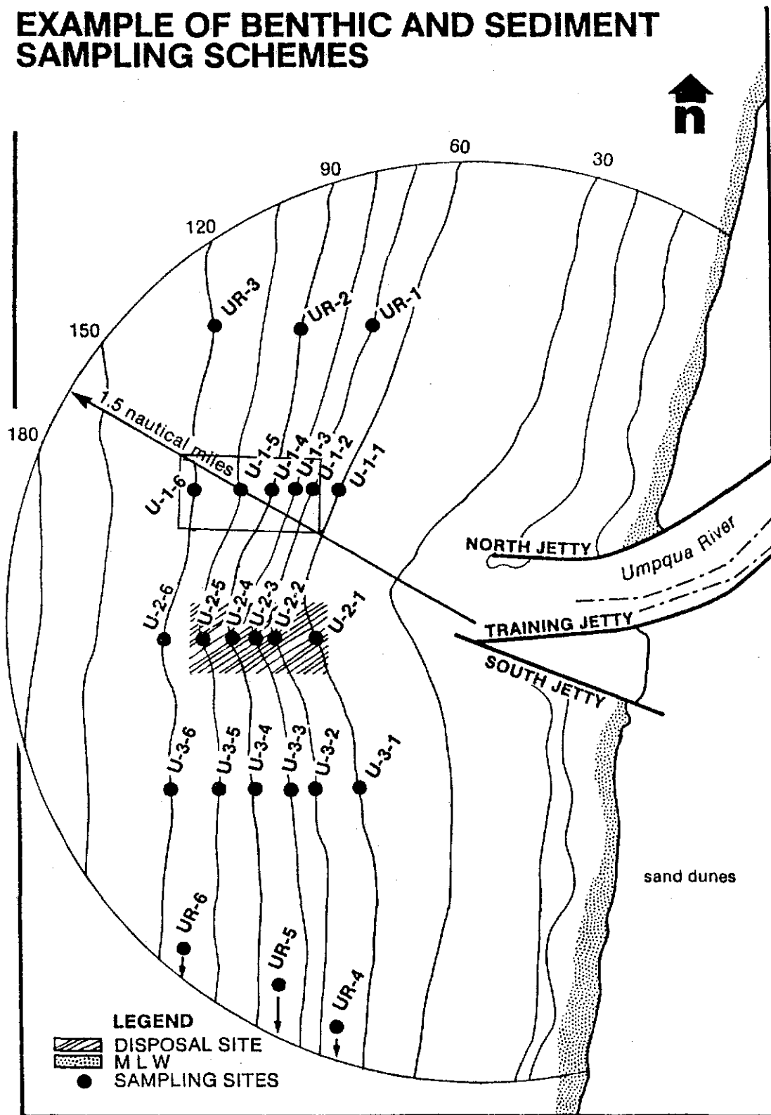
Figure B-3 Umpqua ZSF and sample locations
