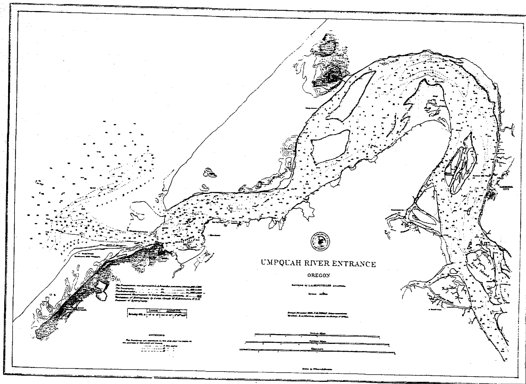
Figure E-1, Umpqua River Entrance in 1887 , (USCGS,1887)
