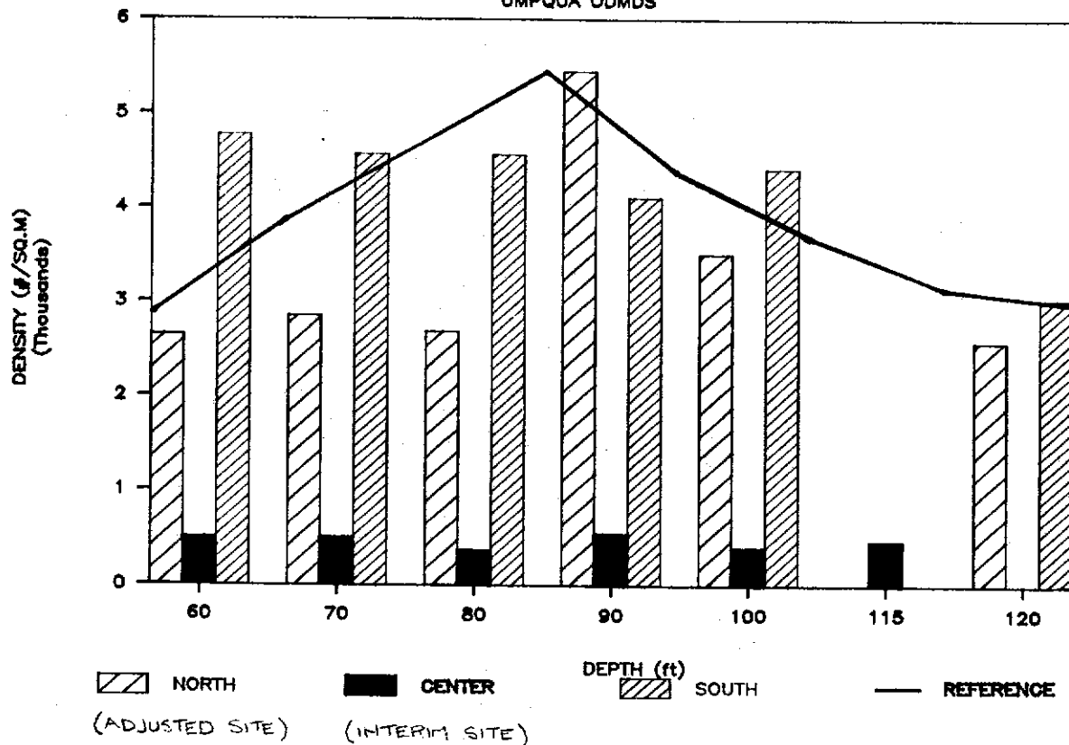
Figure A-2 Density of Benthic Infauna
