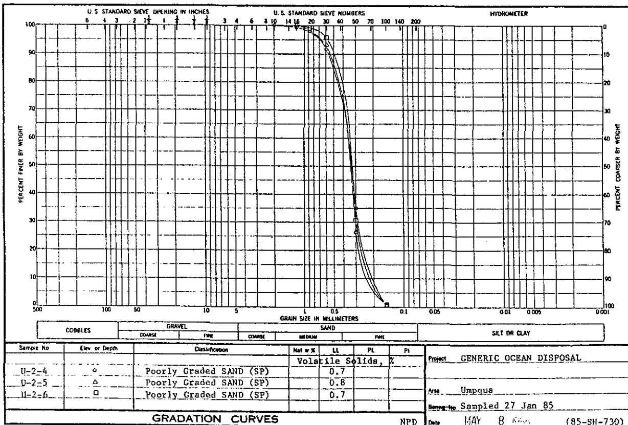
Figure C-9 Gradation Curves
