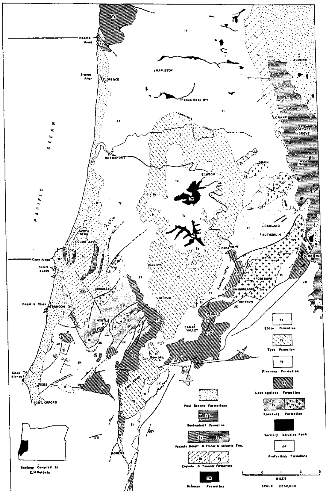
Figure B-2 Coastal Geology near Umpqua
